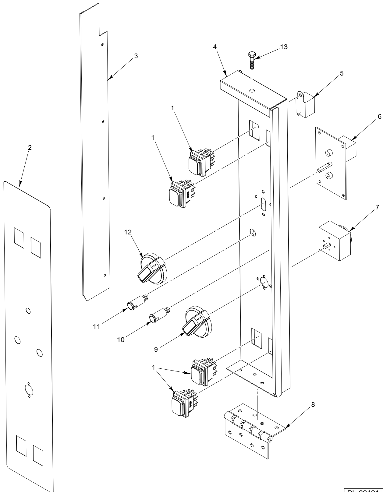
CONTROL PANEL
