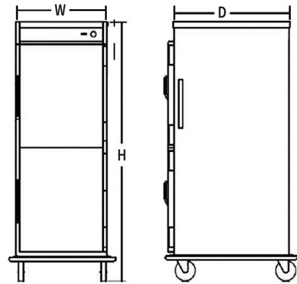
VBP15 & VBP18 Front & Side Views
