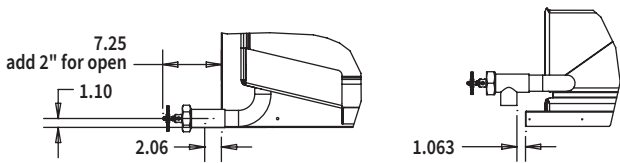
2" Draw-off valve - left front 90° left (BPDV-2)
